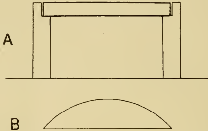
Fig. 340. A, Span of proposed bridge. B, Stress diagram, or diagram of bending-moments*.
