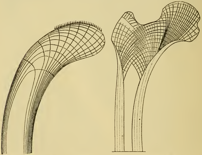
Fig. 335. Crane-head and femur. (After Culmann and H. Meyer.)
