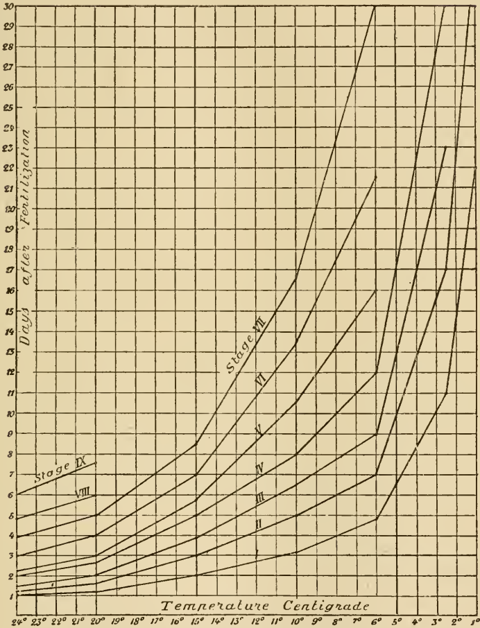
Fig. 28. Diagram shewing time taken (in days), at various temperatures (°C.), to reach certain stages of development in the Frog: viz. I, gastrula; II, medullary plate; III, closure of medullary folds; IV, tail-bud; V, tail and gills; VI, tail-fin; VII, operculum beginning; VIII, do. closing; IX, first appearance of hind-legs. (From Jenkinson, after O. Hertwig, 1898.)
