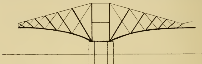
Fig. 345. A two-armed cantilever of the Forth Bridge. Thick lines, compression-members (bones); thin lines, tension-members (ligaments).
