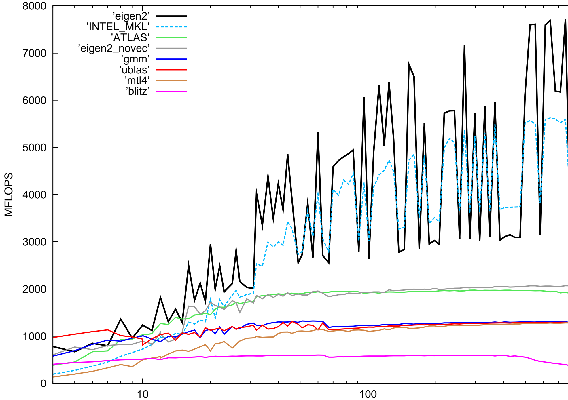
transposed-matrix vector product
